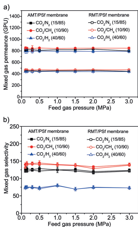
Figure 5. a) CO 2 permeance and b) selectivity of the AMT/PSf (filled symbols) and RMT/PSf (open symbols) membranes tested with gas mixtures. AMT/PSf has a much higher gas permeance than RMT/PSf, but a similar gas pair selectivity.
